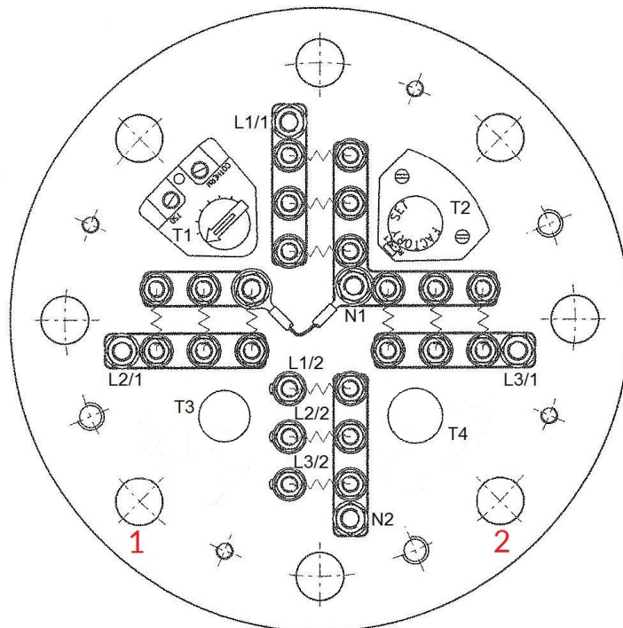
Terminal Layout
