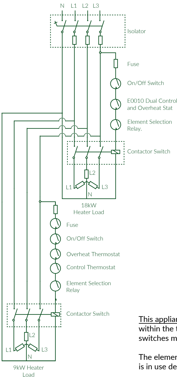
Wiring Diagram
