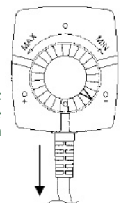
Right: Correct installation features the cable facing vertically down
